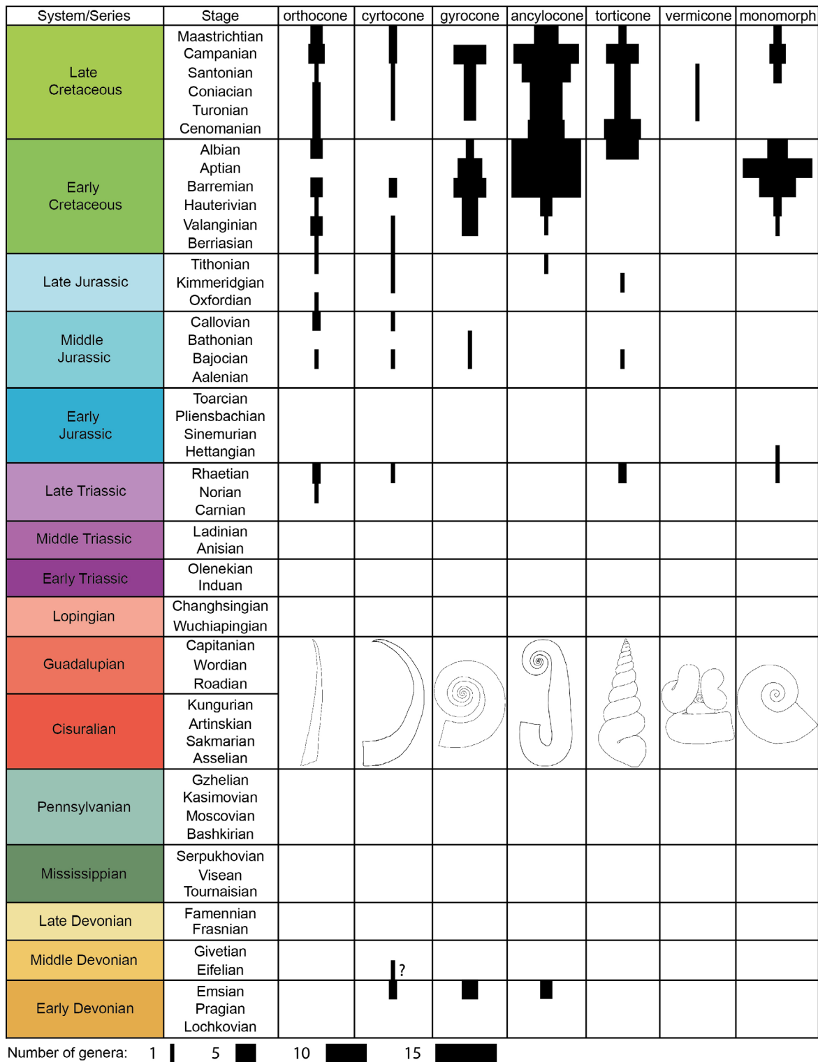
Fig. 11. Stratigraphic distribution of the six arche-morphotypes of heteromorphous conchs from the Devonian, Triassic, Jurassic, and Cretaceous. Also shown are secondarily monomorphous forms derived from heteromorphs. After Wright et al. (1996).
