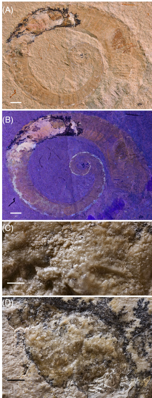
Fig. 6. Stomach content of Allocioceras (specimen shown in Wippich & Lehmann, 2004). (A) Image taken under daylight. (B) Same specimen imaged under ultraviolet light showing preserved soft parts such as the siphuncle and remnants of the stomach. (C) Close up of assumed but unidentifiable stomach remains. (D) Stomach remains of planktic comatolids (crinoids). Scale bars: A and B = 5 mm, C and D = 0.5 mm.
