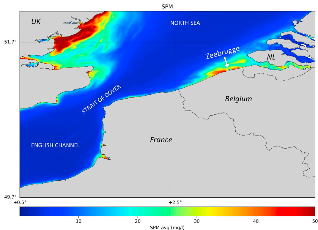
Fig. 1. Near surface sediment concentrations in the English Channel and southern North Sea, revealing elevated SSC near Zeebrugge computed from satellite images covering the period 2003–2011 and using the algorithms of Nechad et al. (2010).
