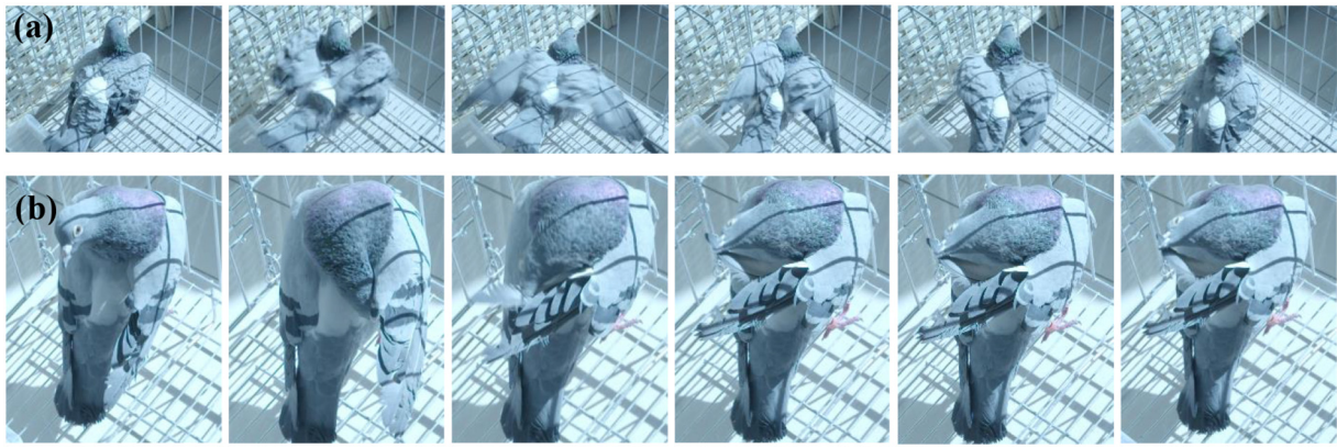
Fig. 1. Domestic pigeon recovers its messy feathers. (a) Shaking the wings to recover the ruffled feathers. When detecting that the barbules of a feather are split, the pigeon first shakes its wings to recover them. After shaking the wings several times, most of the feather vanes are recovered to their normal state. Only a small number of vanes remain in a mess. (b) Preening the ruffled feathers. After detecting some feathers are still in a mess, the pigeon uses its beak to preen the split barbules from the root to the distal of the vane. The pigeon often repeats this process with its beak until the feathers are completely recovered.
