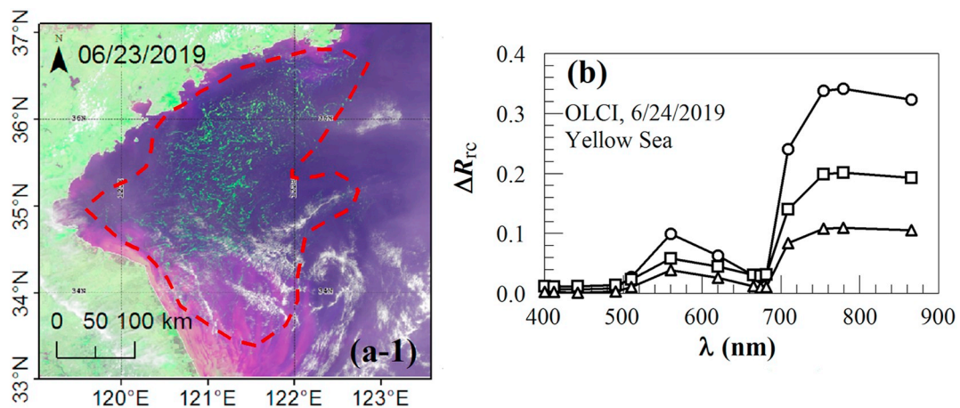
Fig. 3. (a) VIIRS FRGB image shows an Ulva bloom in the western Yellow Sea (Box 3 in Fig. 1 & Table 2). (b) Typical OLCI \Delta R_{rc}(\lambda) of several pixels selected from the greenish image features. (For interpretation of the references to color in this figure legend, the reader is referred to the web version of this article.)
