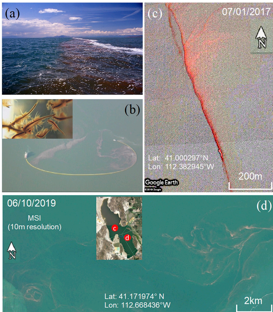
Fig. 12. (a) Surface aggregation of brine shrimp ( Artemia ) eggs in the Great Salt Lake (photo taken by Gilbert Bay on 24 June 2009); (b) An airborne photo shows corralling of brine shrimp eggs for harvesting (photo courtesy of https://saltlakebrineshrimp.com/harvest/ ). The inset figure shows the brine shrimp, with an average length of ~0.7–1.3 cm for adults. (c) Google Earth image on 1 July 2017 shows surface aggregation of brine shrimp eggs in the Great Salt Lake. (d) MSI true-color RGB image on 10 June 2019 shows image slicks where the spectral shapes appear to be similar to those of Fig. 11b, therefore possibly caused by aggregations of brine shrimp eggs. The inset map shows the locations of (c) & (d) in the Great Salt Lake.
