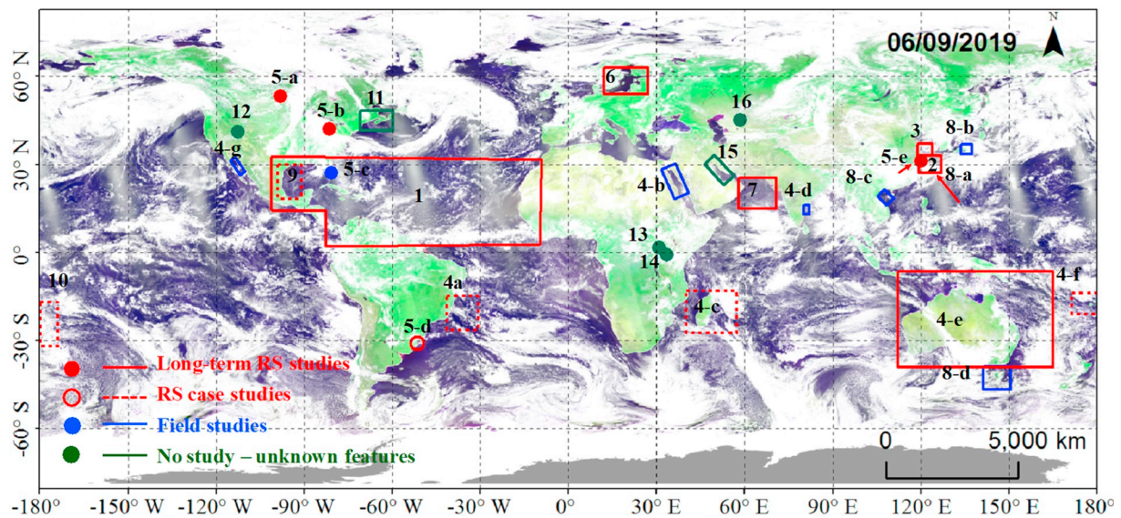
Fig. 1. Distribution of floating algae and floating organisms/materials around the world, obtained from inspections of VIIRS FRGB images available through NOAA OCView. The known and unknown features are color coded, with more details provided in Table 2.
