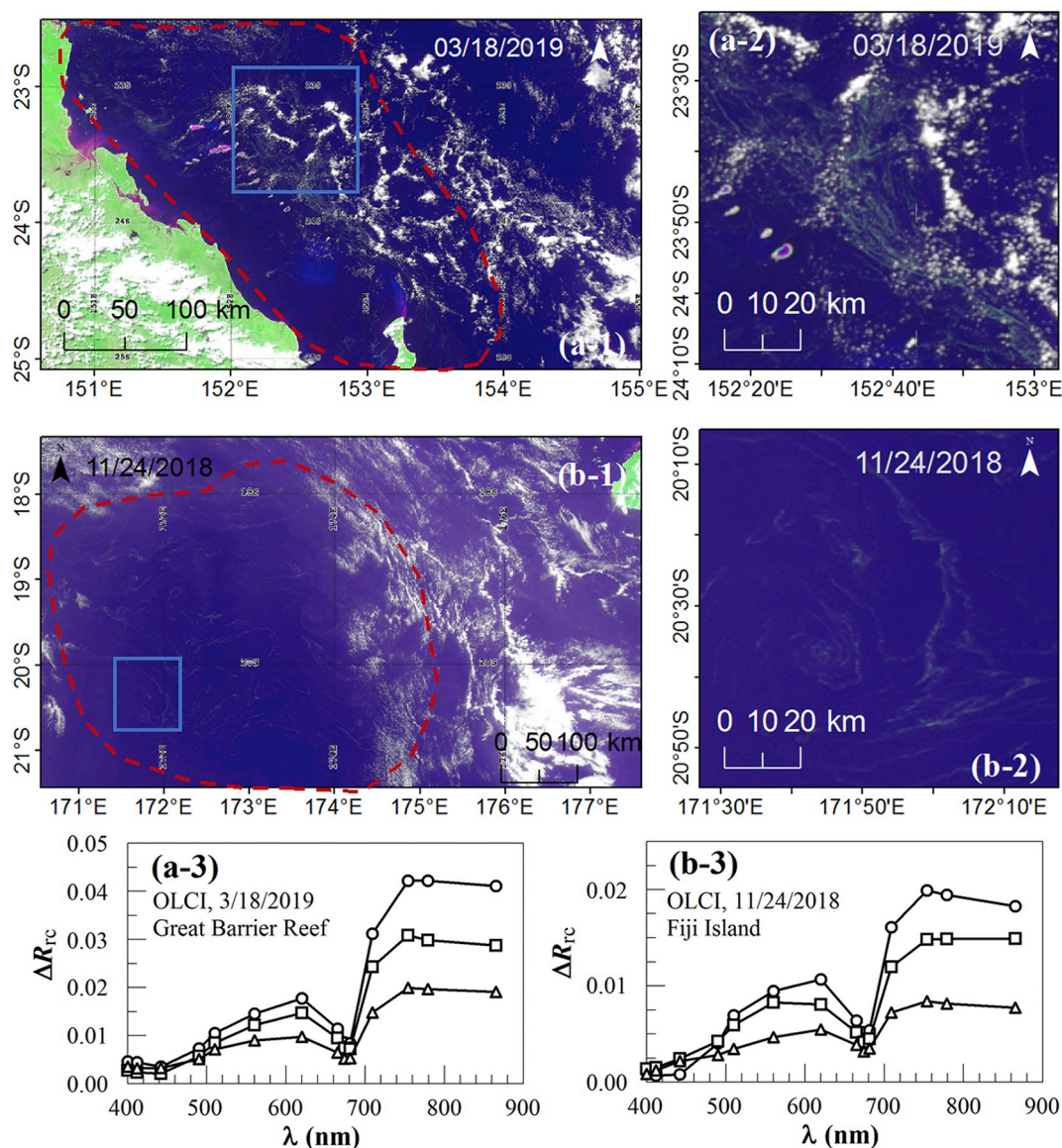
Fig. 5. VIIRS FRGB images show Trichodesmium blooms (a-1) around Great Barrier Reef off east coast of Australia, (b-1) around Fiji island in the South Pacific, (c-1) near Madagascar, and (d-1) in the South Atlantic Ocean east of the southwest Brazil. The areal extents of algae slicks are outlined in red, and the image features from the small squares are enlarged to the right. The OLCI-derived \Delta R_{rc}(\lambda) from the slick features are shown in the corresponding figures in (a-3) to (d-3). These features correspond to Boxes 4e, 4f, 4c, and 4a in Fig. 1 & Table 2. (For interpretation of the references to color in this figure legend, the reader is referred to the web version of this article.)
