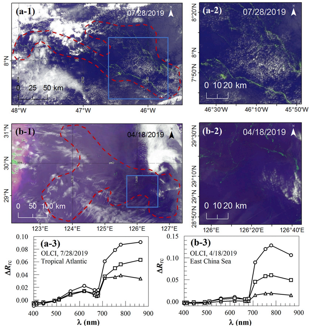
Fig. 2. VIIRS FRGB images show (a) Sargassum fluitans/natans in tropical Atlantic (Box 1 in Fig. 1 & Table 2) and (b) Sargassum horneri in the East China Sea (Box 2 in Fig. 1 & Table 2). From 6 July to 15 August 2019, similar greenish image slicks can be found in all cloud-free and glint-free FRGB images over the same region in (a). The spectra on the bottom represent typical algae spectra extracted from the corresponding OLCI image pixels.
