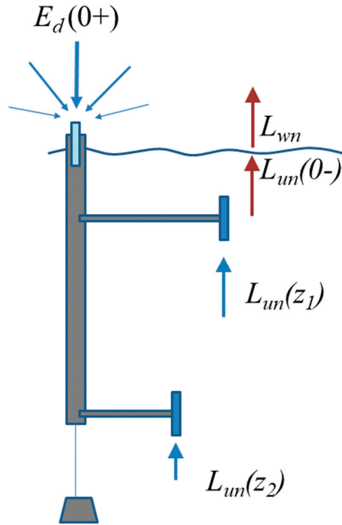
Figure 3. Schematic of fixed-depth underwater measurements.
