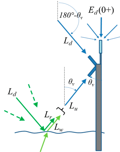
Figure 5. Schematic of above-water radiometry with measurement of sky radiance, L_d , and removal of skylight radiance, L_r . Dashed arrows indicate that contributions to the skylight reflected at the air–water interface come from directions that are not directly measured by the L_d radiance sensor, including possible contributions from the direct sunglint direction.
