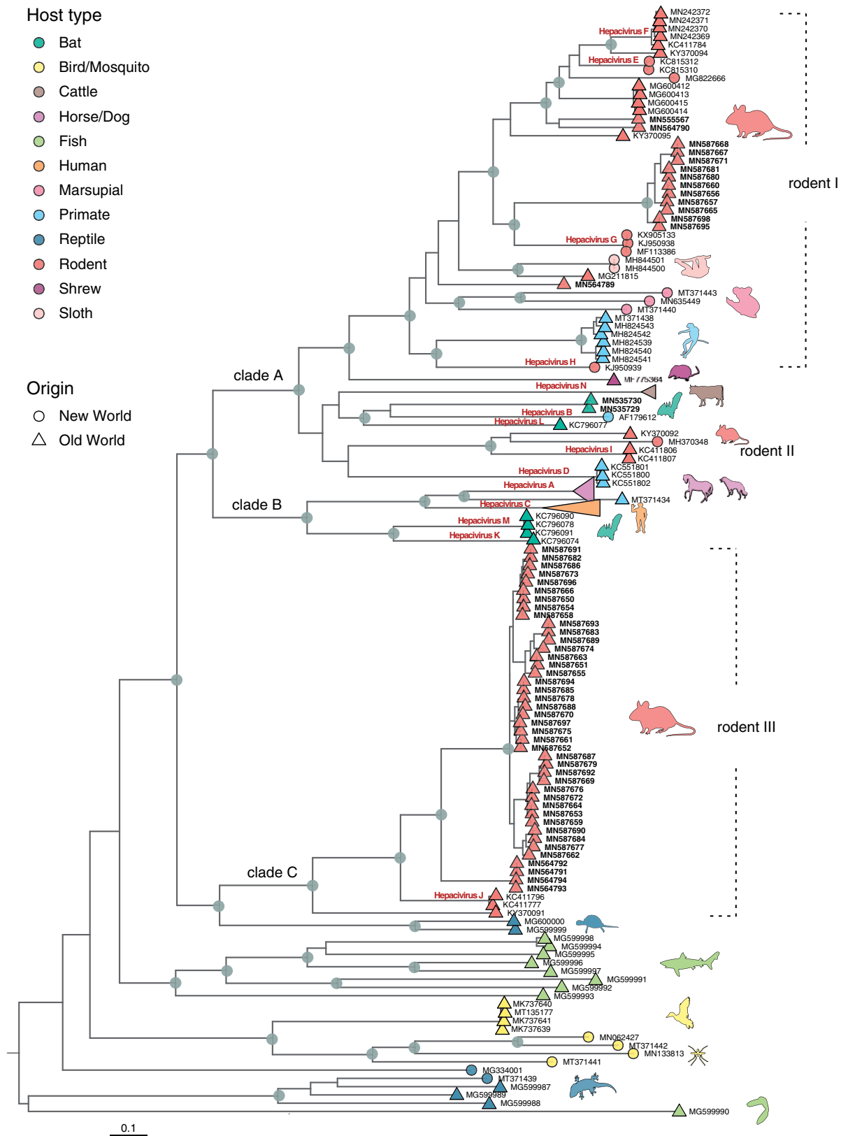
Figure 2. Genome-wide phylogenetic reconstruction of hepatitis C viruses. ML tree of all available ( n=130 ) and novel ( n=58 ) hepatitis C virus genomes. Silhouettes indicate hosts and are coloured according to their broader host type: bats (green), birds and mosquito (yellow), cattles (brown), equids and dog (lilac), fishes (lime green), humans (peach orange), marsupials (pastel pink), primates (light blue), reptiles (steel blue), rodents (salmon), shrew (plum) and sloths (champagne pink). Grey circles indicate internal nodes with bootstrap support \geq 70 , while designated virus species names are shown in bold bordeaux text. Circles at the tips denote New World origin, while triangles represent the Old World viruses. Novel genomes generated in this study are labeled with bold text. Clades A, B and C have been provisionally named for the purpose of discussing the mammalian hepatitis C virus lineages in the main text.
