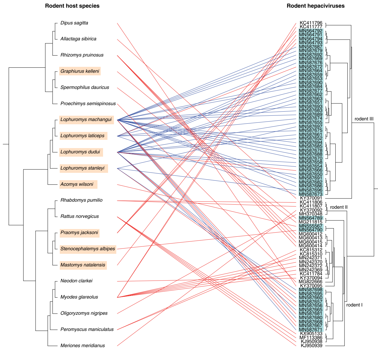
Figure 3. Tanglegram of rodent hosts and their hepatitis C viruses. The topology of the host tree was reconstructed using the cytochrome b gene from twenty-one rodent species (left phylogeny). For the viral reconstruction we used the rodent subset of our genome-wide alignments (right phylogeny) and we highlighted the novel RHV genomes in turquoise. Lines connecting the two phylogenies represent an association between the rodent host species and their identified hepatitis C viruses. Blue lines correspond to individuals harbouring multiple hepatitis C viruses, while rodent species highlighted in a caramel colour represent the novel hosts found to be hepatitis C virus positive.
