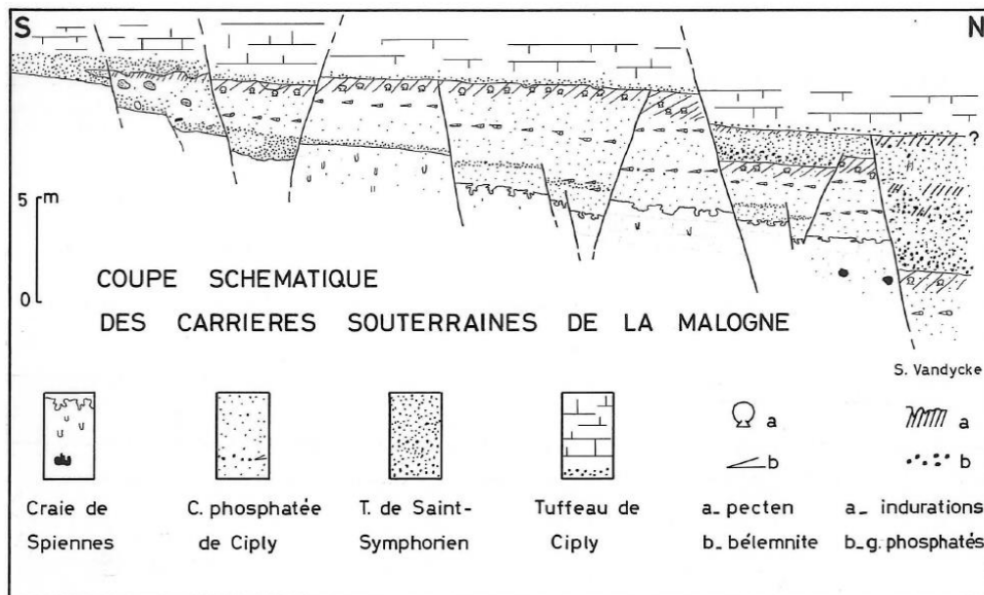
Figure 2: Typical fault pattern in La Malogne underground quarry
