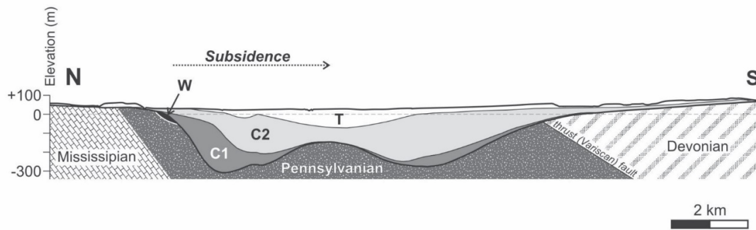
Fig. 2 – Geological cross-section of the Mons Basin in the Bernissart area. The arrow shows the direction of depocenter migration in the northern part of the basin since the Barremian. W: Barremian (Wealden); C1: Albian-Cenomanian ; C2: Turonian-Campanian; T: Tertiary and Quaternary.
