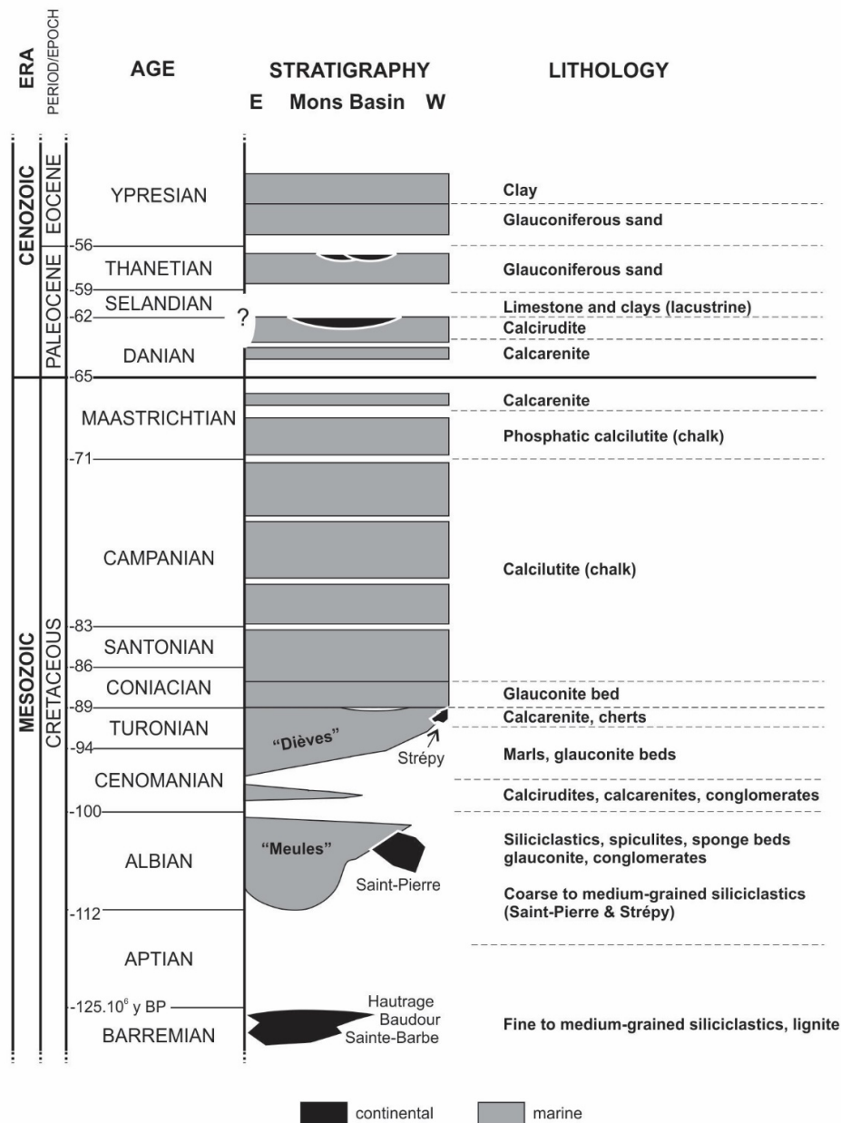
Fig. 3 - Cretaceous lithostratigraphic scale of the Mons Basin (modified after Marlière, 1970 and Robaszynski et al., 2001).
