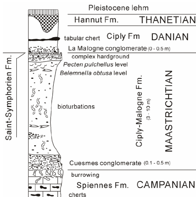
Figure 1: Stratigraphical section in La Malogne underground quarry
