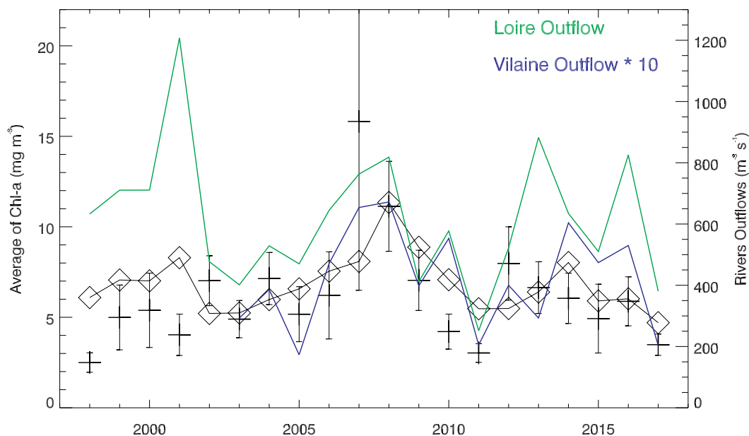
Fig. 12. The averaged satellite (black line and diamonds) and in situ (crosses) Chl- a during the productive season at Ouest_Loscolo in the Vilaine Bay compared to the averaged outflows of the Loire (green) and Vilaine (blue) rivers. The outflows of the Vilaine river are multiplied by 10. (For interpretation of the references to colour in this figure legend, the reader is referred to the web version of this article.)
